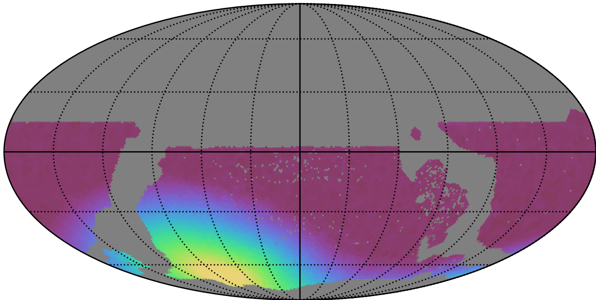
extra_ss_neo4_v3.4_10yrs WFD all bands: Min moonDistance
