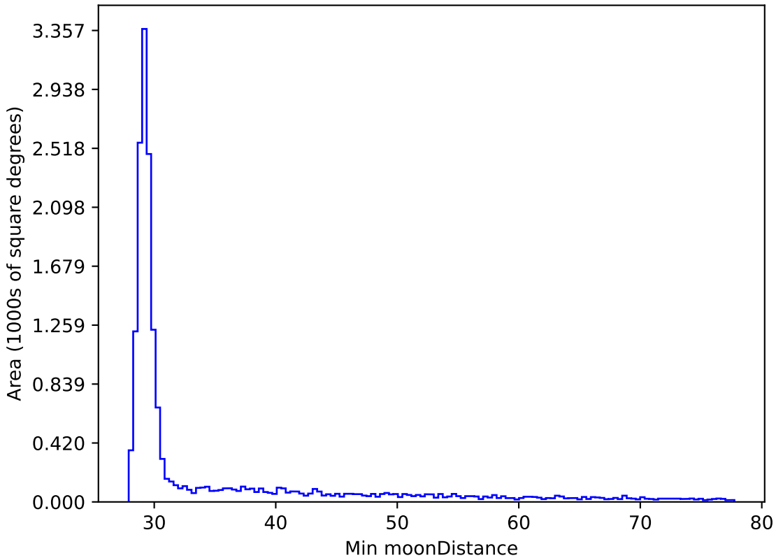
extra_ss_neo4_v3.4_10yrs WFD all bands: Min moonDistance
