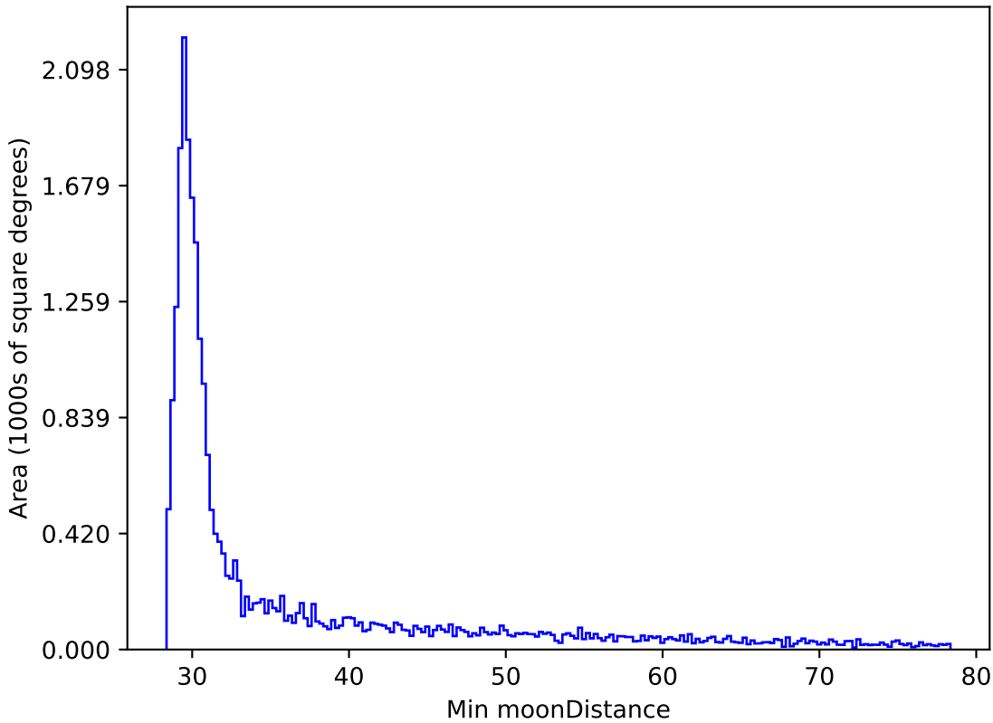
extra_ss_neo4_v3.4_10yrs All sky z band: Min moonDistance
