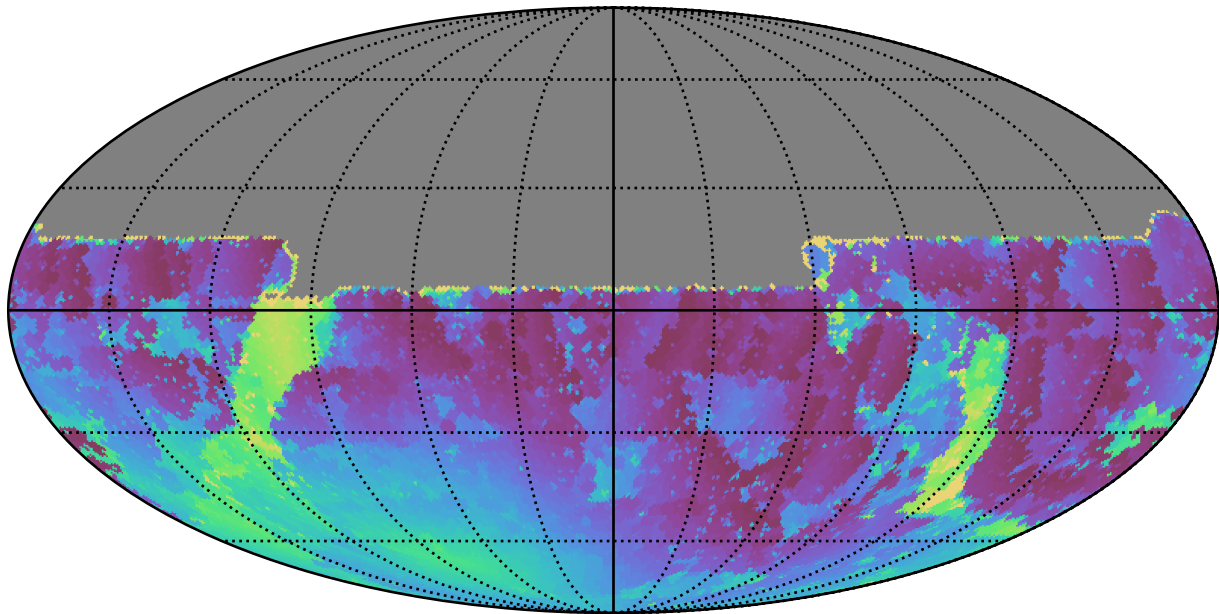
extra_ss_neo4_v3.4_10yrs All sky u band: Min moonDistance
