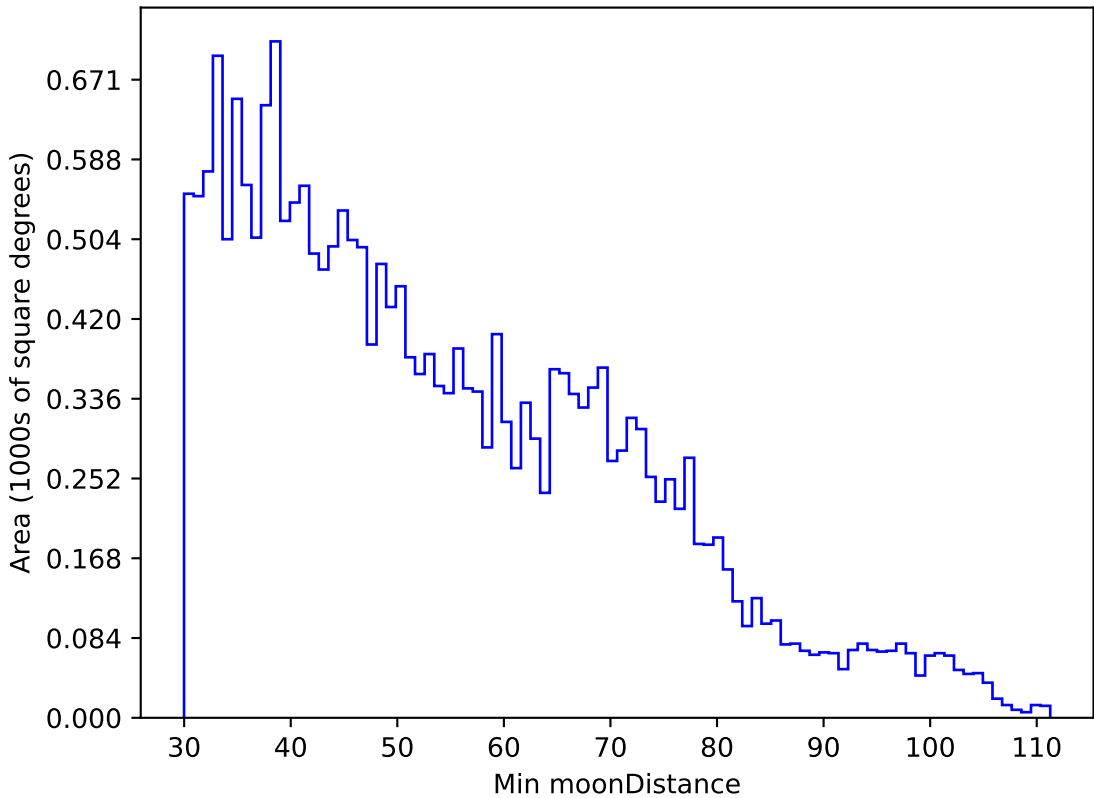
extra_ss_neo4_v3.4_10yrs All sky u band: Min moonDistance
