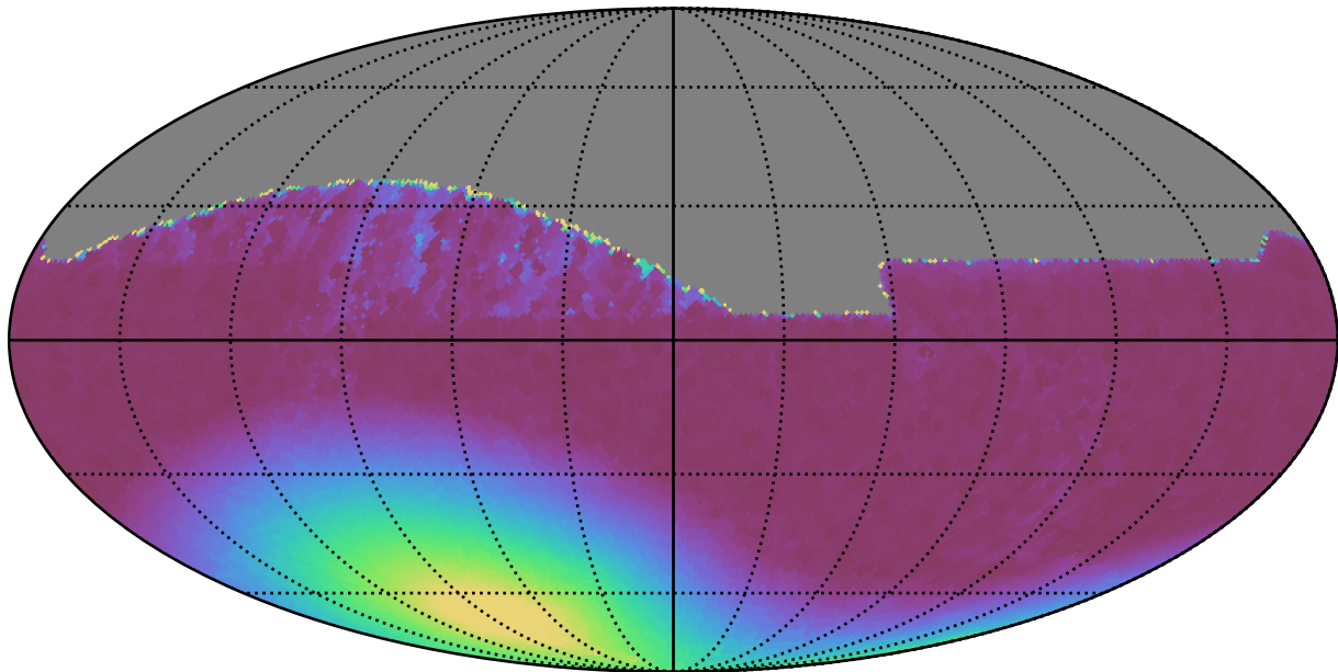
extra_ss_neo4_v3.4_10yrs All sky all bands: Min moonDistance
