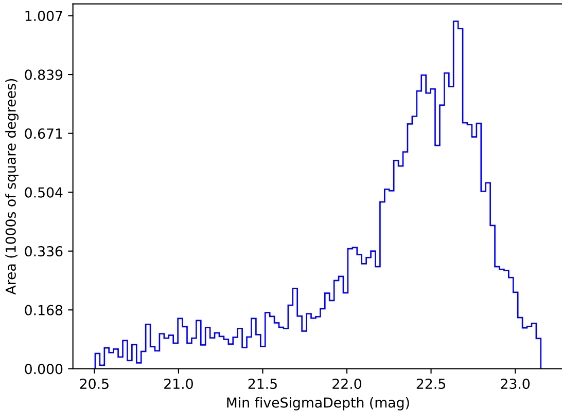
extra_ss_neo4_v3.4_10yrs Yr 1 z band: Min fiveSigmaDepth
