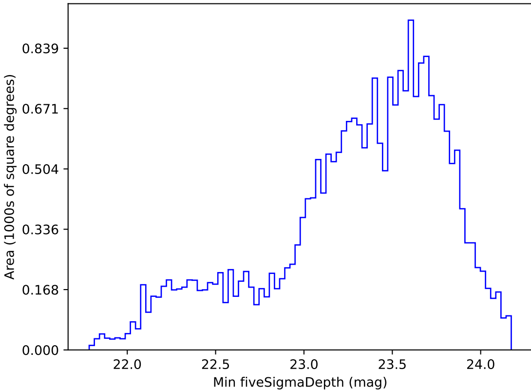
extra_ss_neo4_v3.4_10yrs Yr 1 r band: Min fiveSigmaDepth
