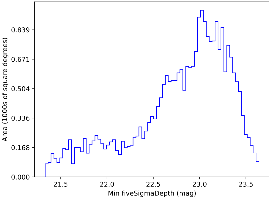
extra_ss_neo4_v3.4_10yrs Yr 1 i band: Min fiveSigmaDepth
