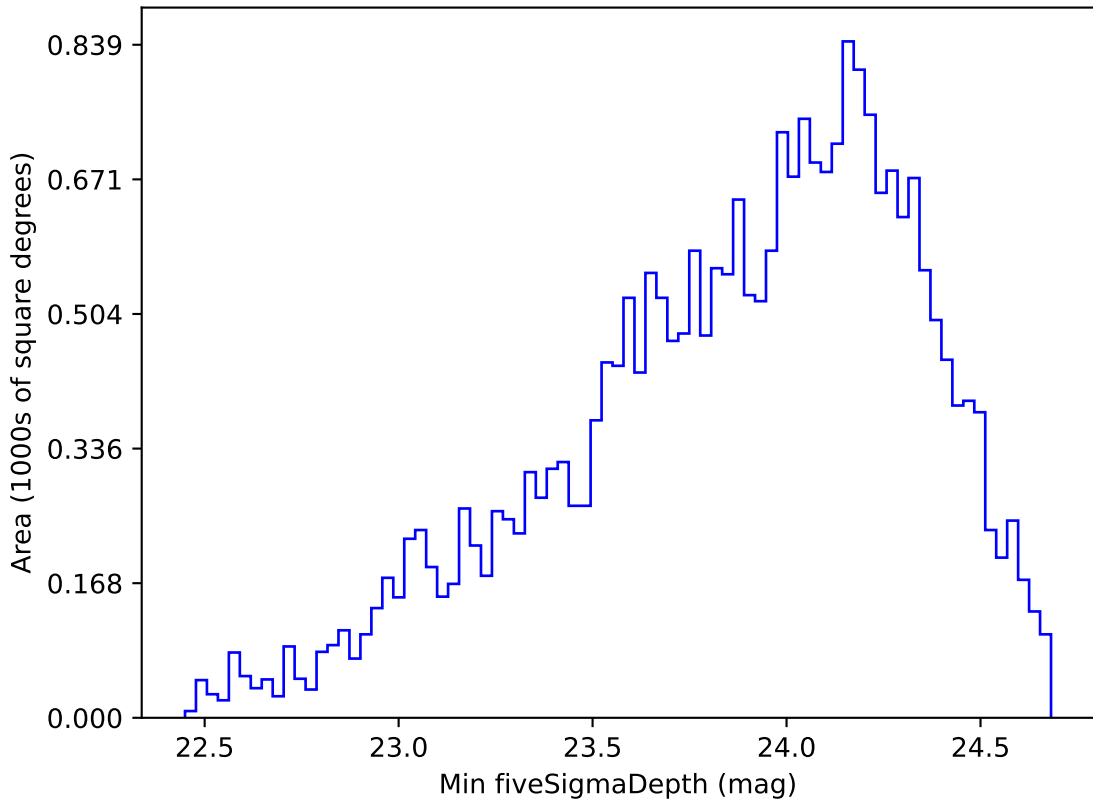
extra_ss_neo4_v3.4_10yrs Yr 1 g band: Min fiveSigmaDepth
