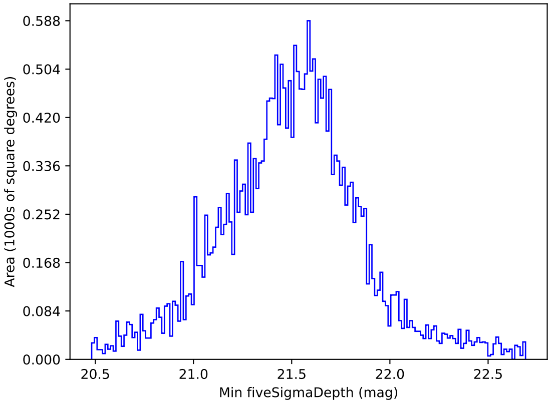
extra_ss_neo4_v3.4_10yrs Yr 1 all bands: Min fiveSigmaDepth
