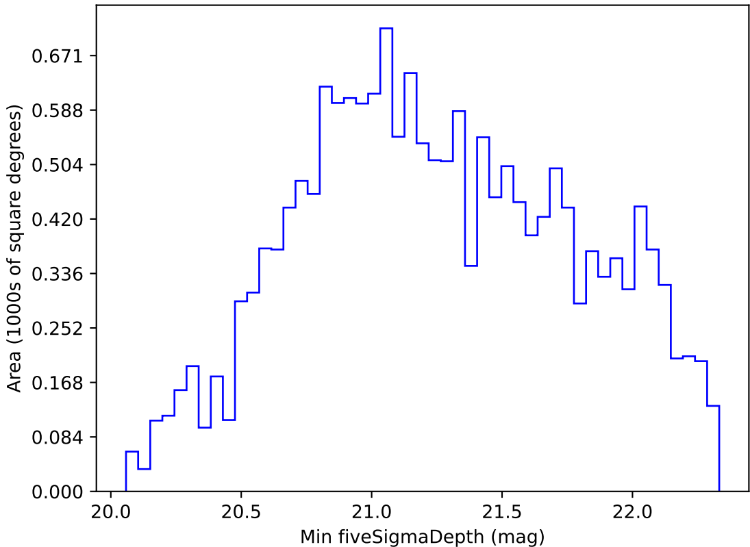
extra_ss_neo4_v3.4_10yrs WFD z band: Min fiveSigmaDepth
