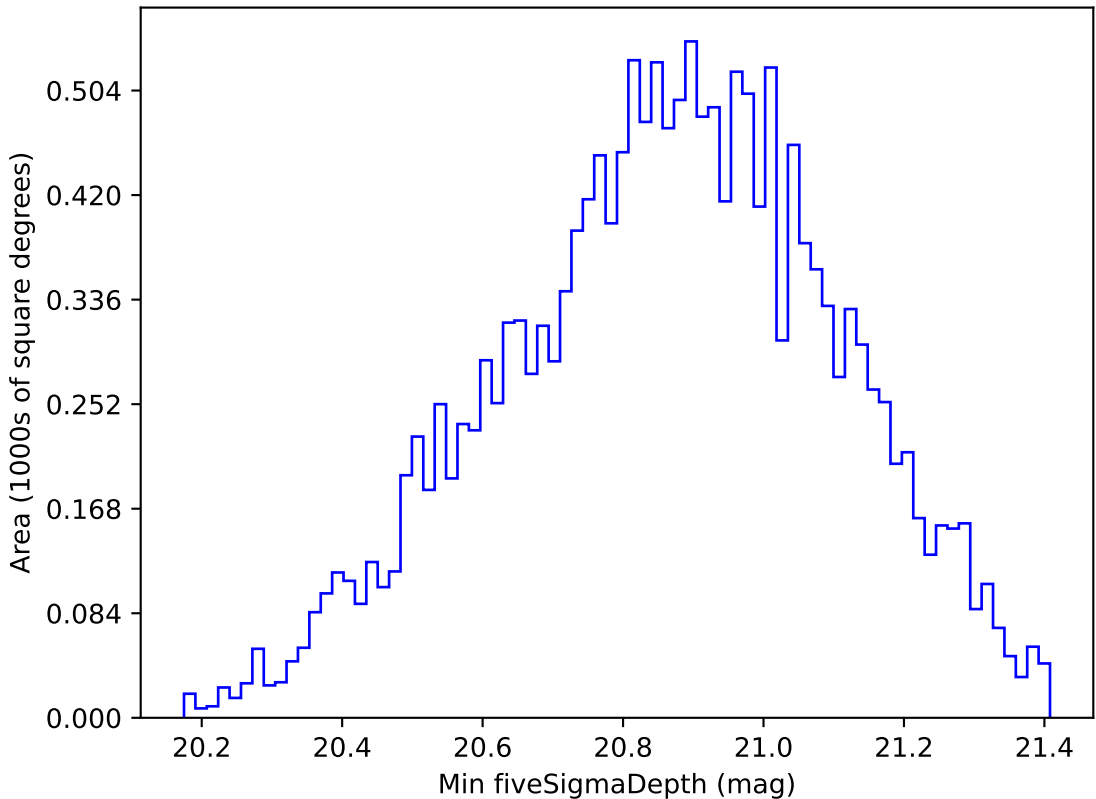
extra_ss_neo4_v3.4_10yrs WFD y band: Min fiveSigmaDepth
