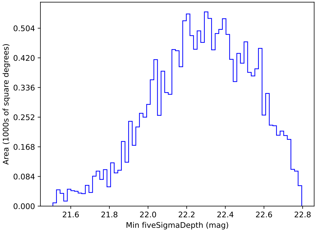
extra_ss_neo4_v3.4_10yrs WFD u band: Min fiveSigmaDepth
