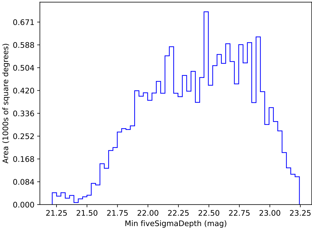
extra_ss_neo4_v3.4_10yrs WFD r band: Min fiveSigmaDepth
