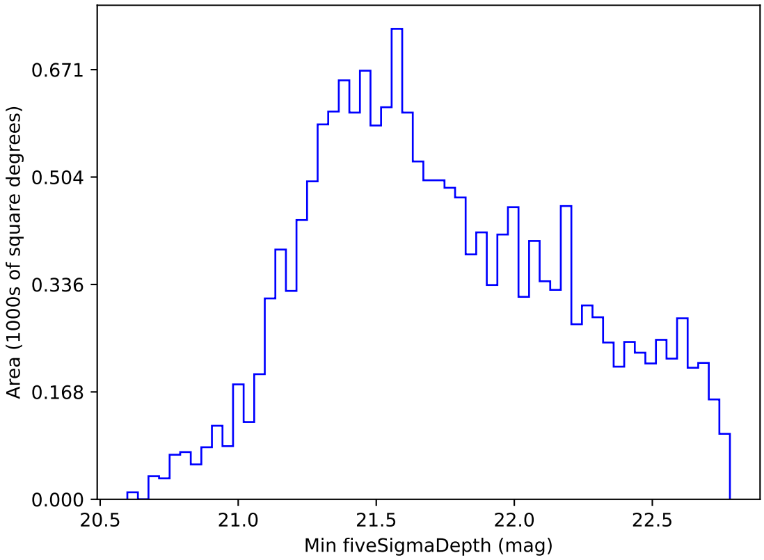
extra_ss_neo4_v3.4_10yrs WFD i band: Min fiveSigmaDepth
