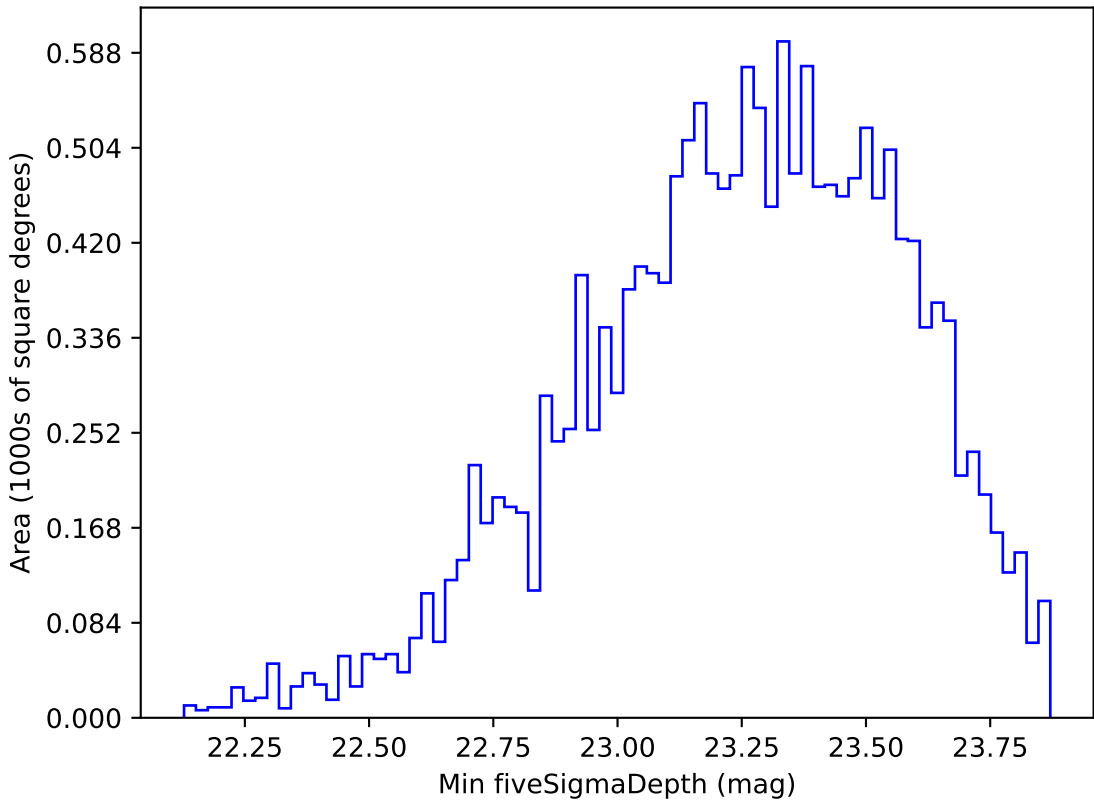
extra_ss_neo4_v3.4_10yrs WFD g band: Min fiveSigmaDepth
