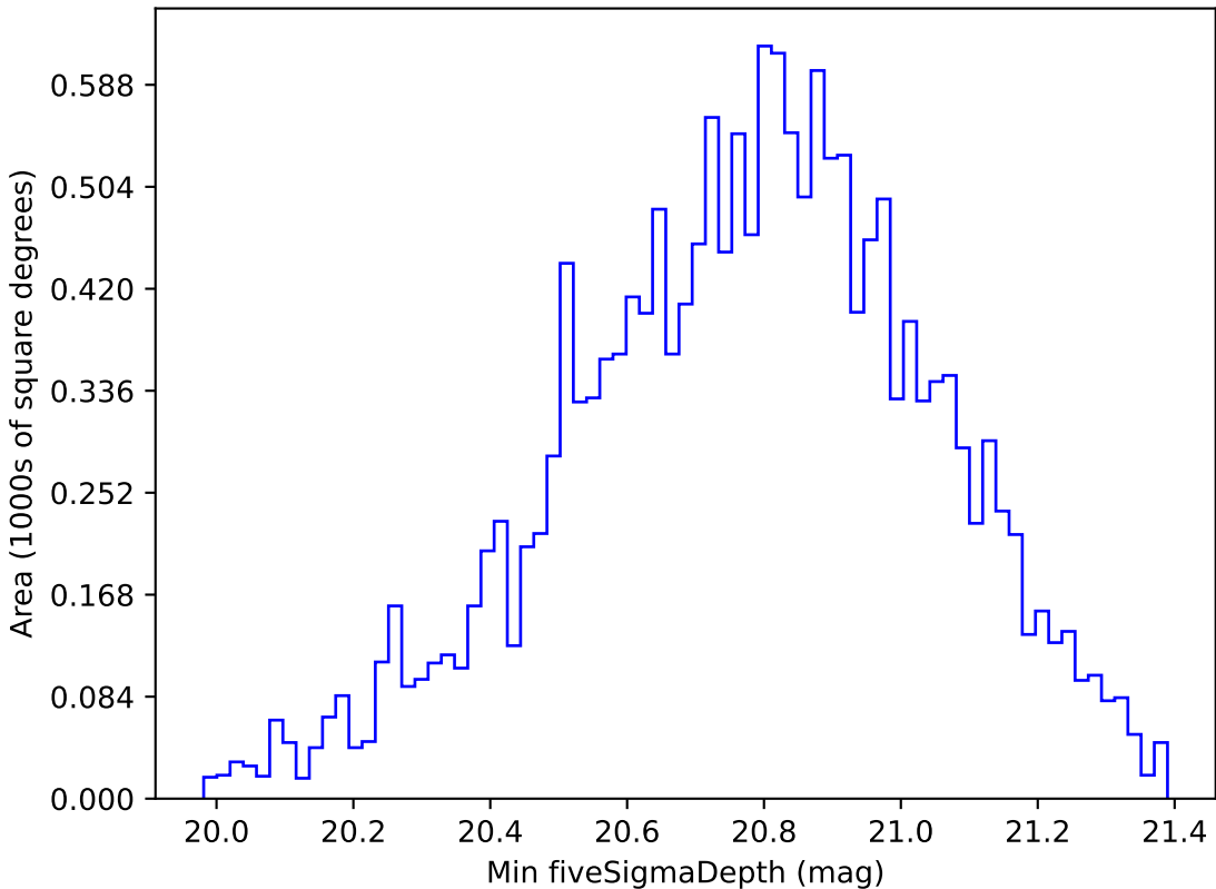
extra_ss_neo4_v3.4_10yrs WFD all bands: Min fiveSigmaDepth
