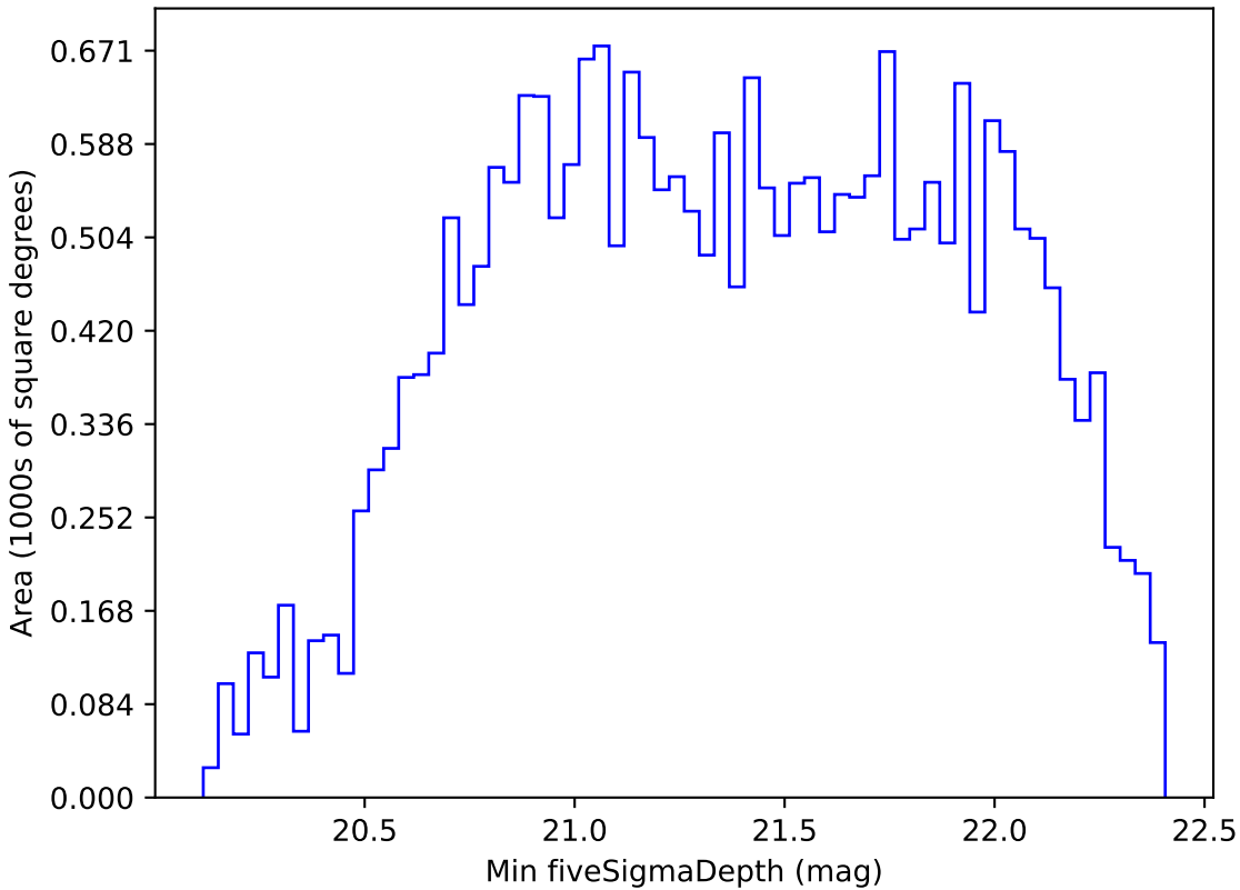
extra_ss_neo4_v3.4_10yrs All sky z band: Min fiveSigmaDepth
