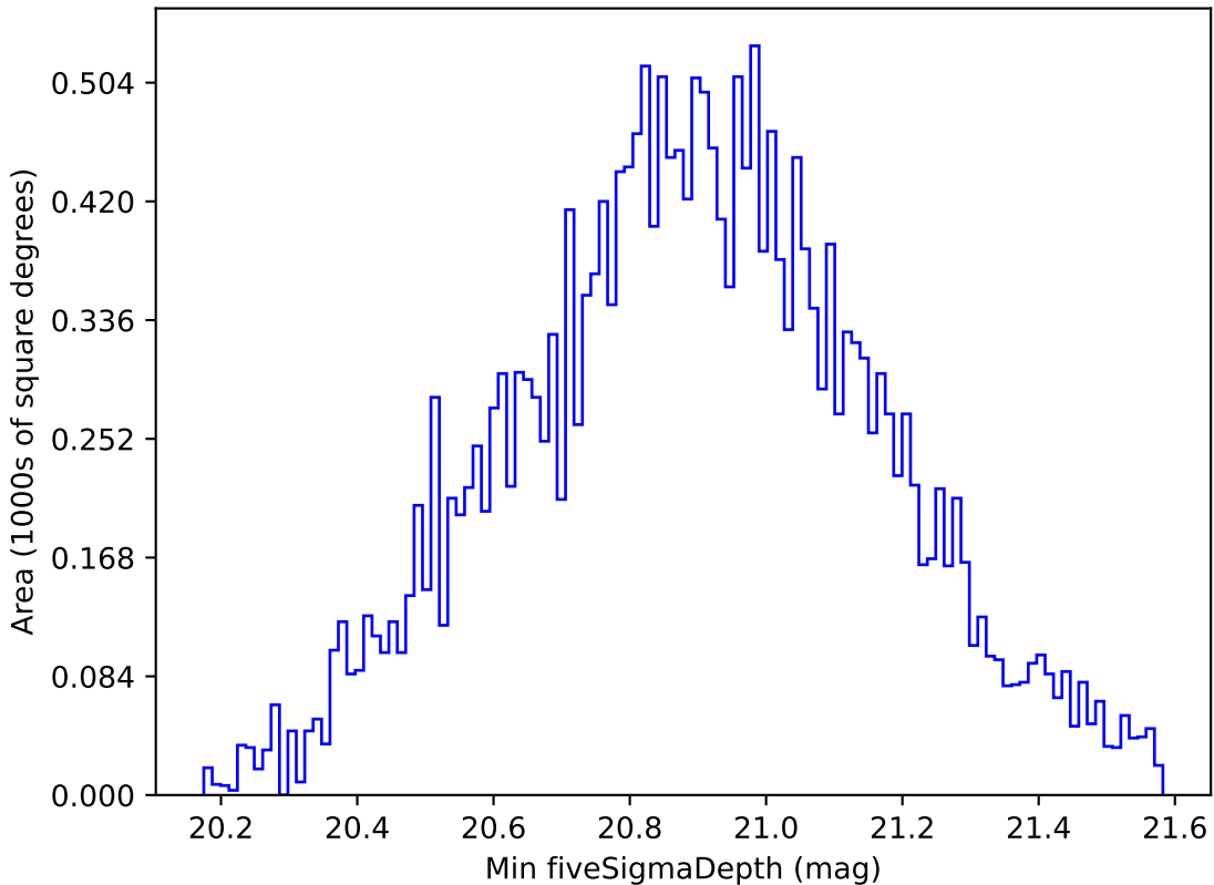
extra_ss_neo4_v3.4_10yrs All sky y band: Min fiveSigmaDepth
