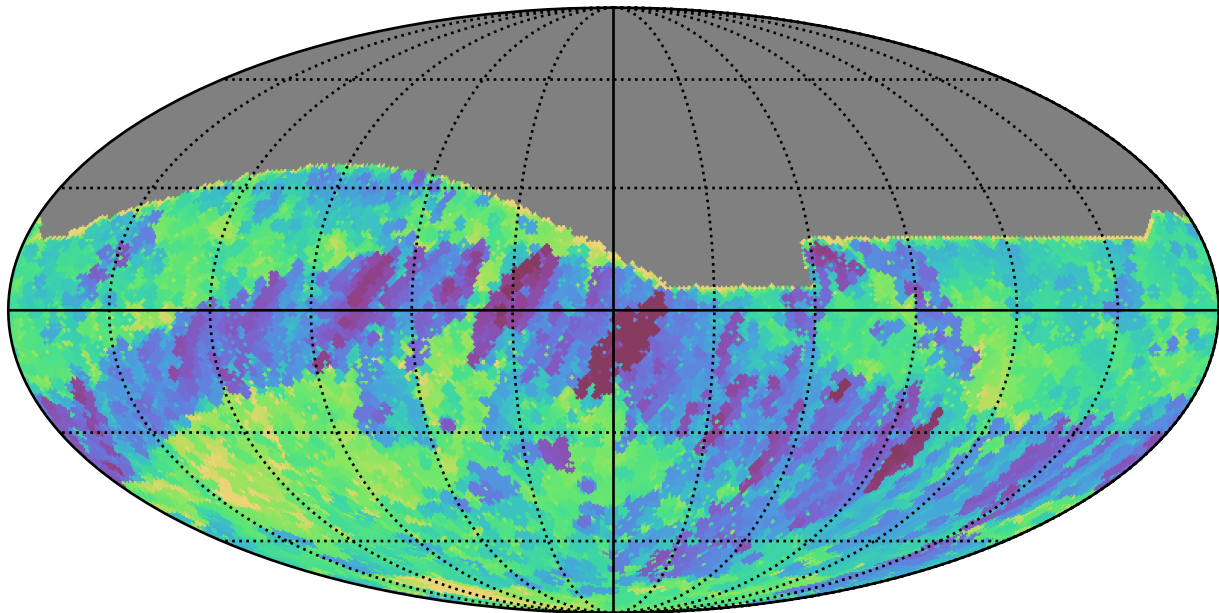
extra_ss_neo4_v3.4_10yrs All sky r band: Min fiveSigmaDepth
