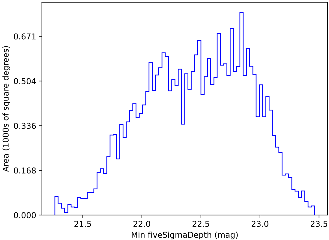
extra_ss_neo4_v3.4_10yrs All sky r band: Min fiveSigmaDepth
