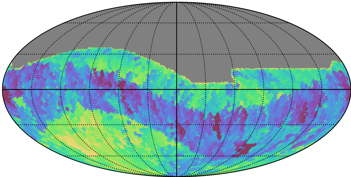
extra_ss_neo4_v3.4_10yrs All sky i band: Min fiveSigmaDepth
