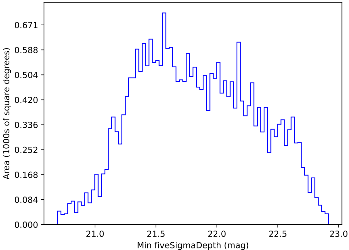
extra_ss_neo4_v3.4_10yrs All sky i band: Min fiveSigmaDepth
