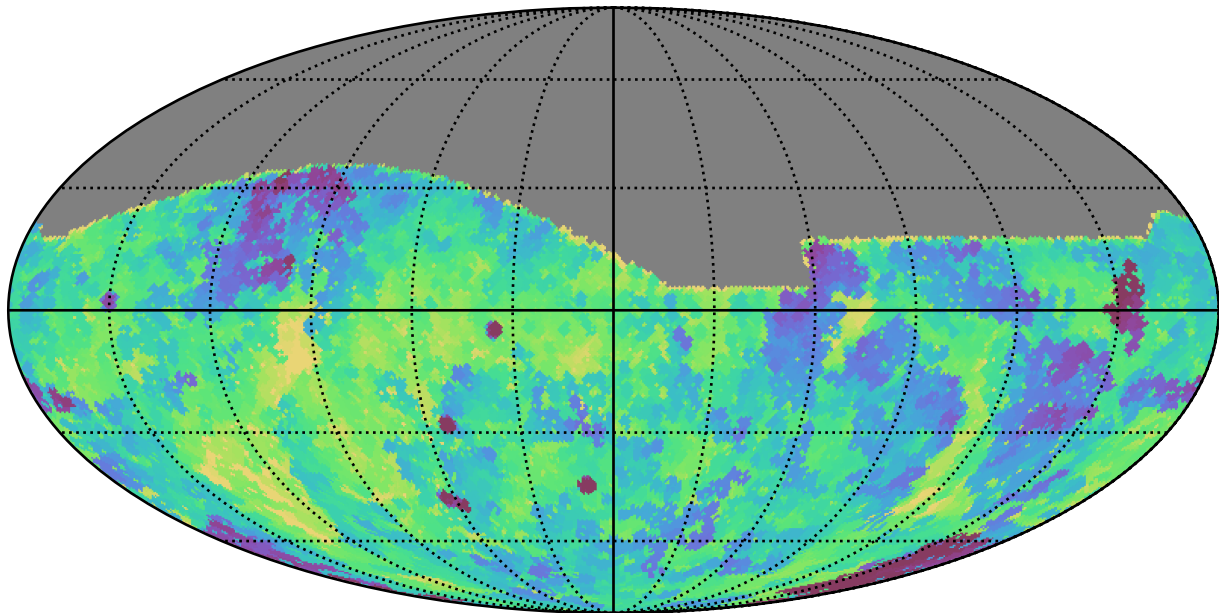
extra_ss_neo4_v3.4_10yrs All sky g band: Min fiveSigmaDepth
