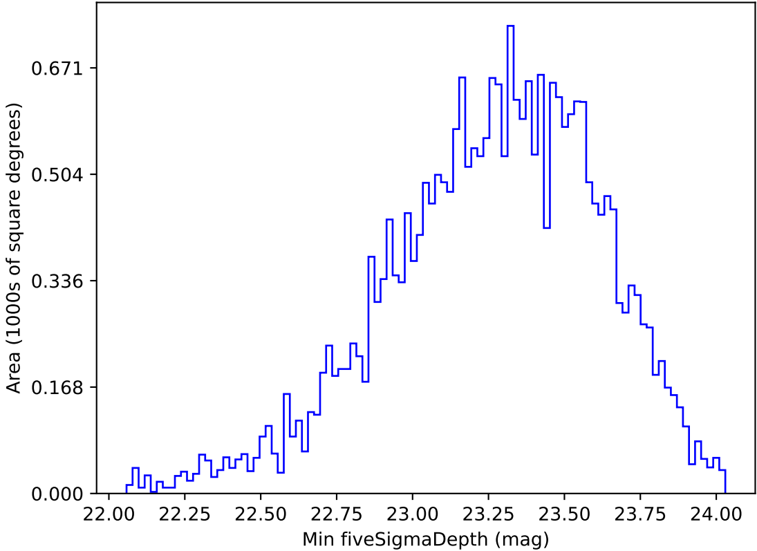
extra_ss_neo4_v3.4_10yrs All sky g band: Min fiveSigmaDepth
