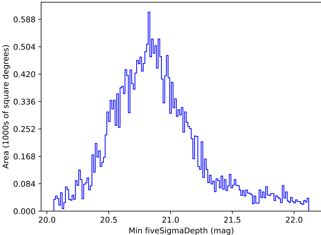
extra_ss_neo4_v3.4_10yrs All sky all bands: Min fiveSigmaDepth
