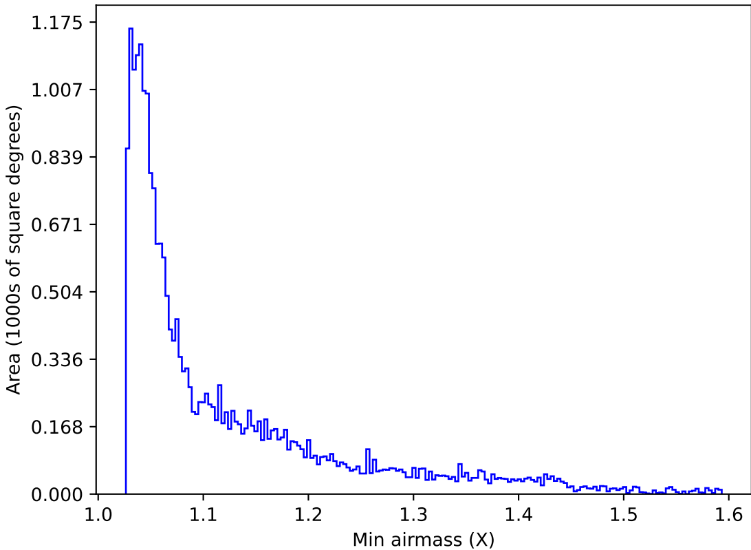
extra_ss_neo4_v3.4_10yrs Yr 1 y band: Min airmass
