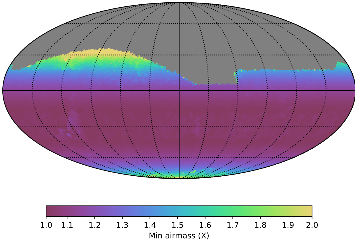
extra_ss_neo4_v3.4_10yrs Yr 1 r band: Min airmass
