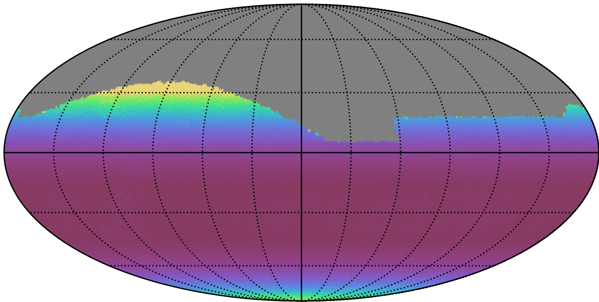
extra_ss_neo4_v3.4_10yrs Yr 1 all bands: Min airmass
