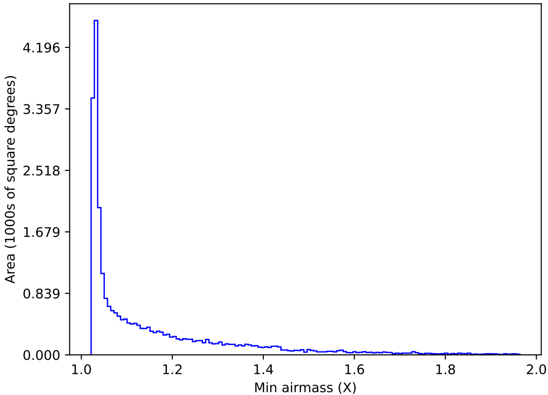
extra_ss_neo4_v3.4_10yrs Yr 1 all bands: Min airmass
