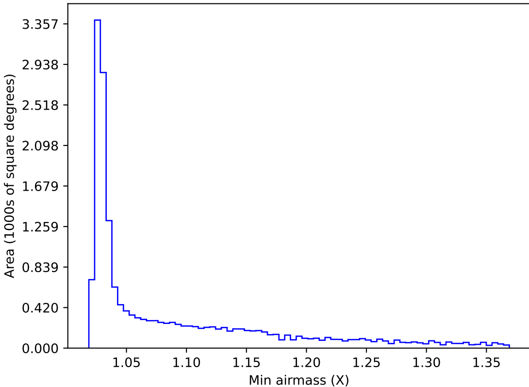
extra_ss_neo4_v3.4_10yrs WFD z band: Min airmass
