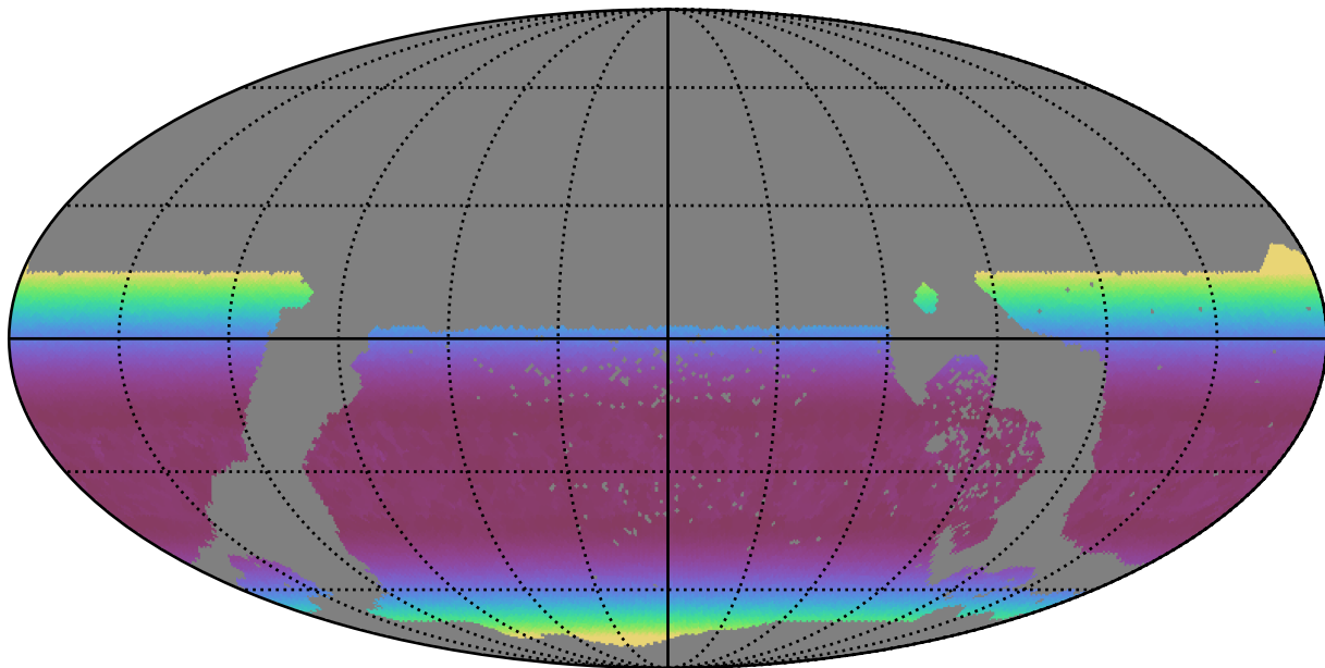
extra_ss_neo4_v3.4_10yrs WFD y band: Min airmass
