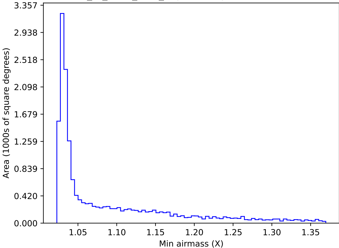
extra_ss_neo4_v3.4_10yrs WFD y band: Min airmass
