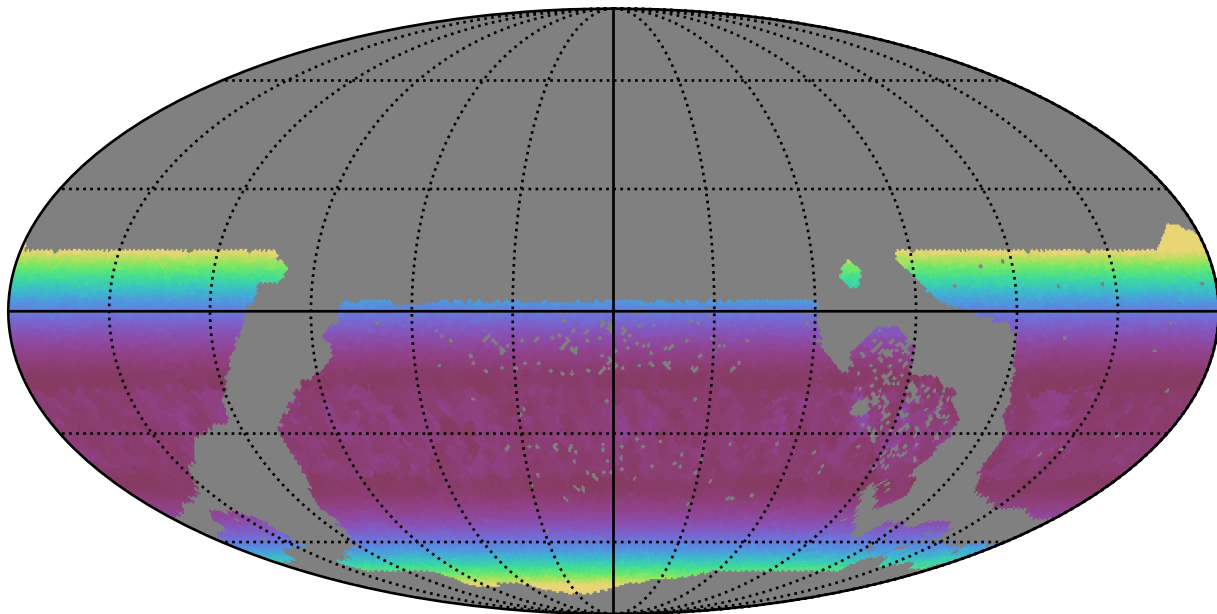
extra_ss_neo4_v3.4_10yrs WFD u band: Min airmass
