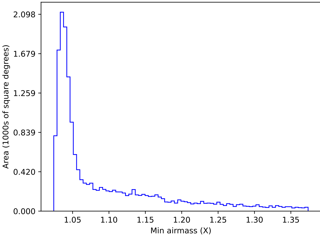
extra_ss_neo4_v3.4_10yrs WFD u band: Min airmass
