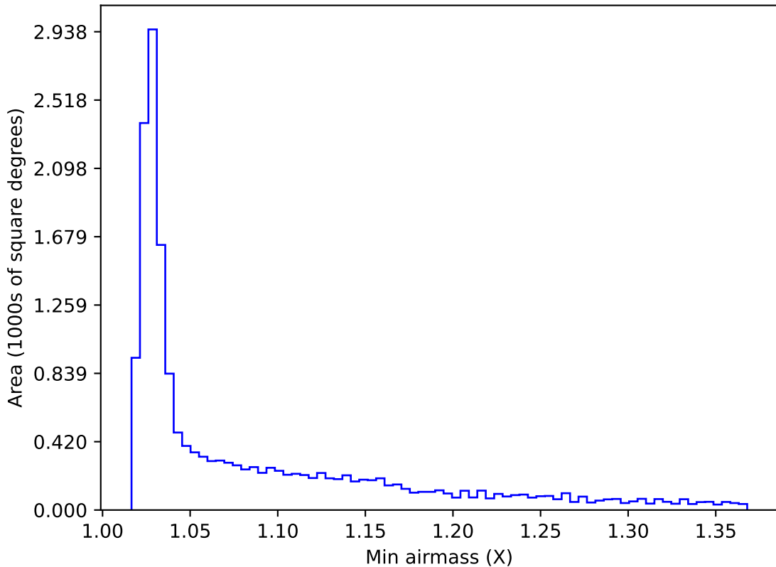
extra_ss_neo4_v3.4_10yrs WFD r band: Min airmass
