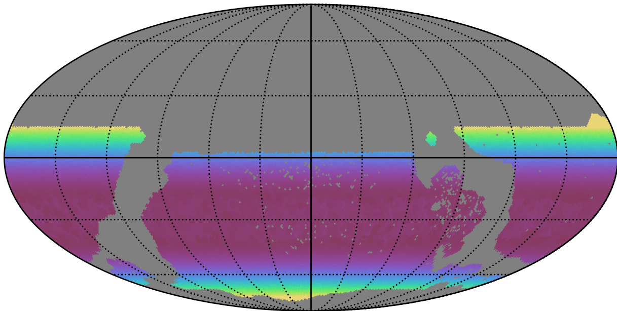
extra_ss_neo4_v3.4_10yrs WFD i band: Min airmass
