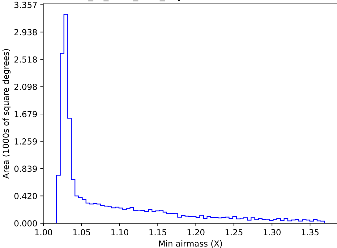
extra_ss_neo4_v3.4_10yrs WFD i band: Min airmass
