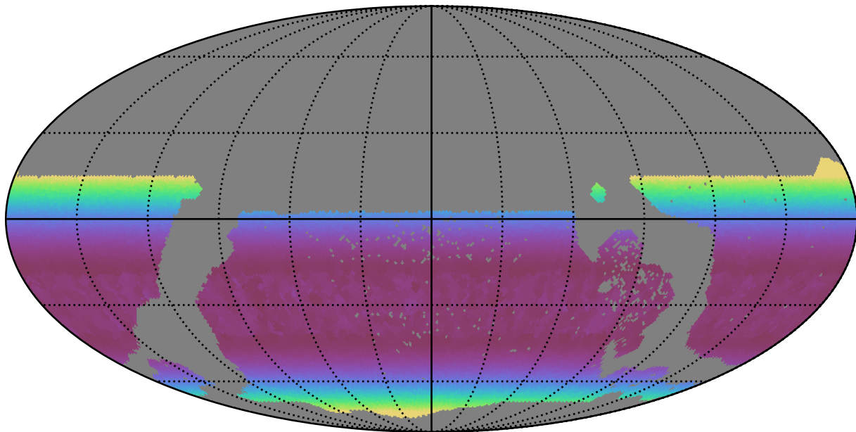
extra_ss_neo4_v3.4_10yrs WFD g band: Min airmass
