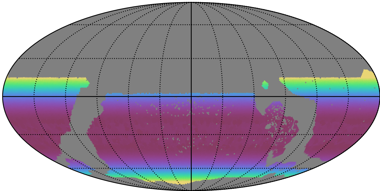
extra_ss_neo4_v3.4_10yrs WFD all bands: Min airmass
