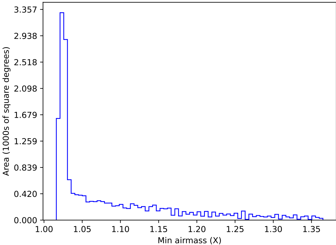
extra_ss_neo4_v3.4_10yrs WFD all bands: Min airmass
