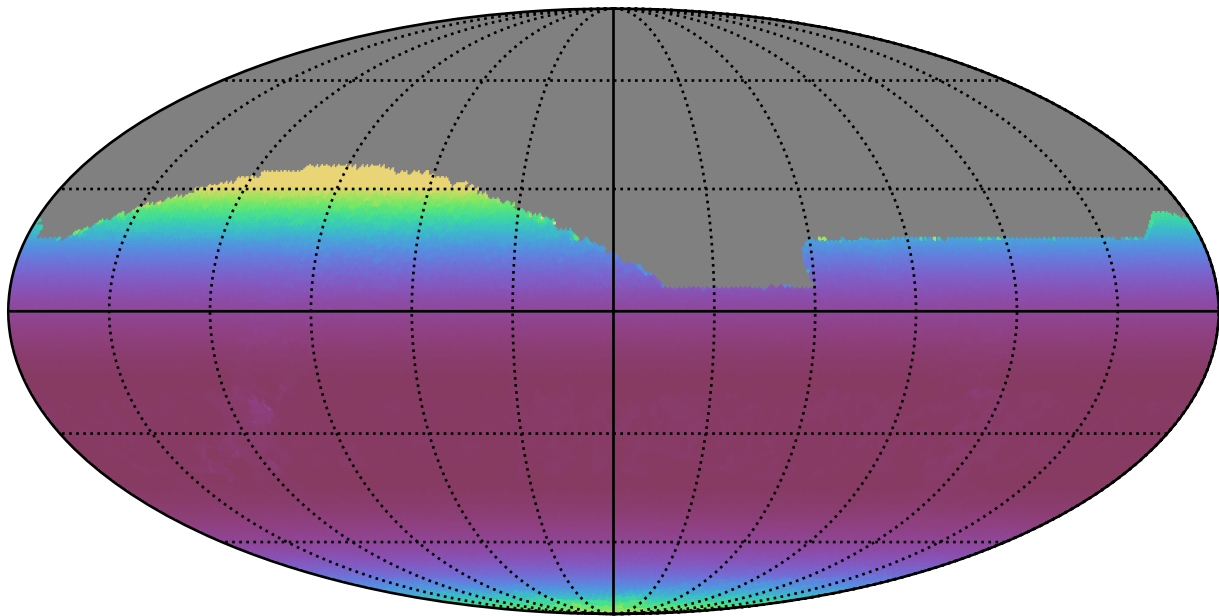
extra_ss_neo4_v3.4_10yrs All sky z band: Min airmass
