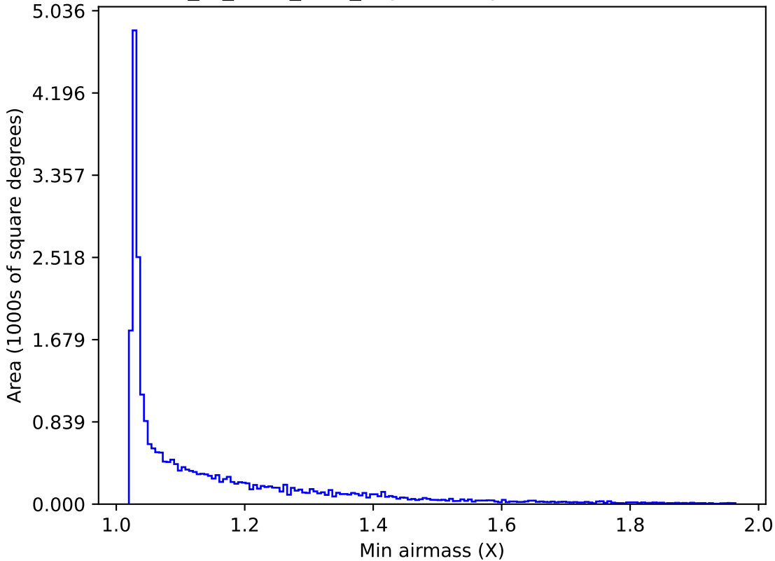
extra_ss_neo4_v3.4_10yrs All sky z band: Min airmass
