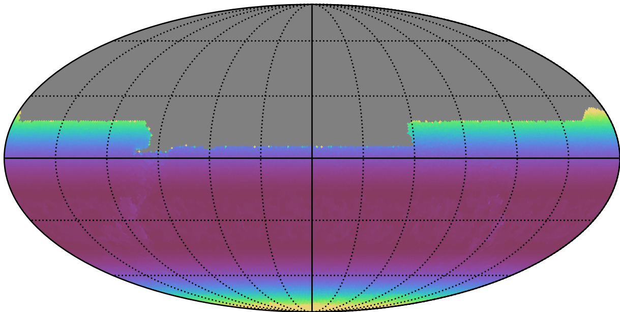
extra_ss_neo4_v3.4_10yrs All sky y band: Min airmass
