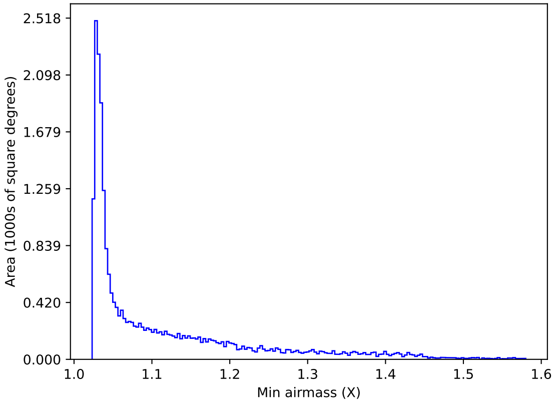
extra_ss_neo4_v3.4_10yrs All sky y band: Min airmass
