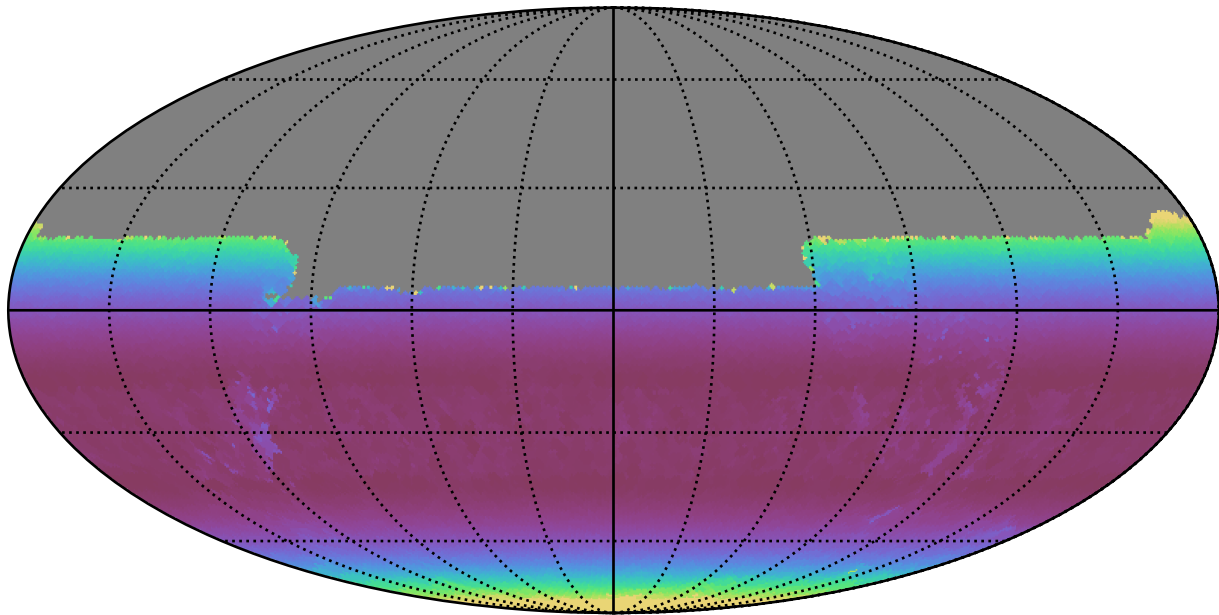
extra_ss_neo4_v3.4_10yrs All sky u band: Min airmass
