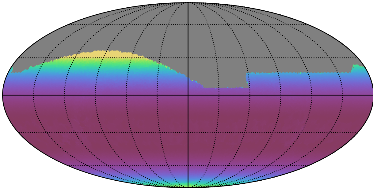
extra_ss_neo4_v3.4_10yrs All sky i band: Min airmass
