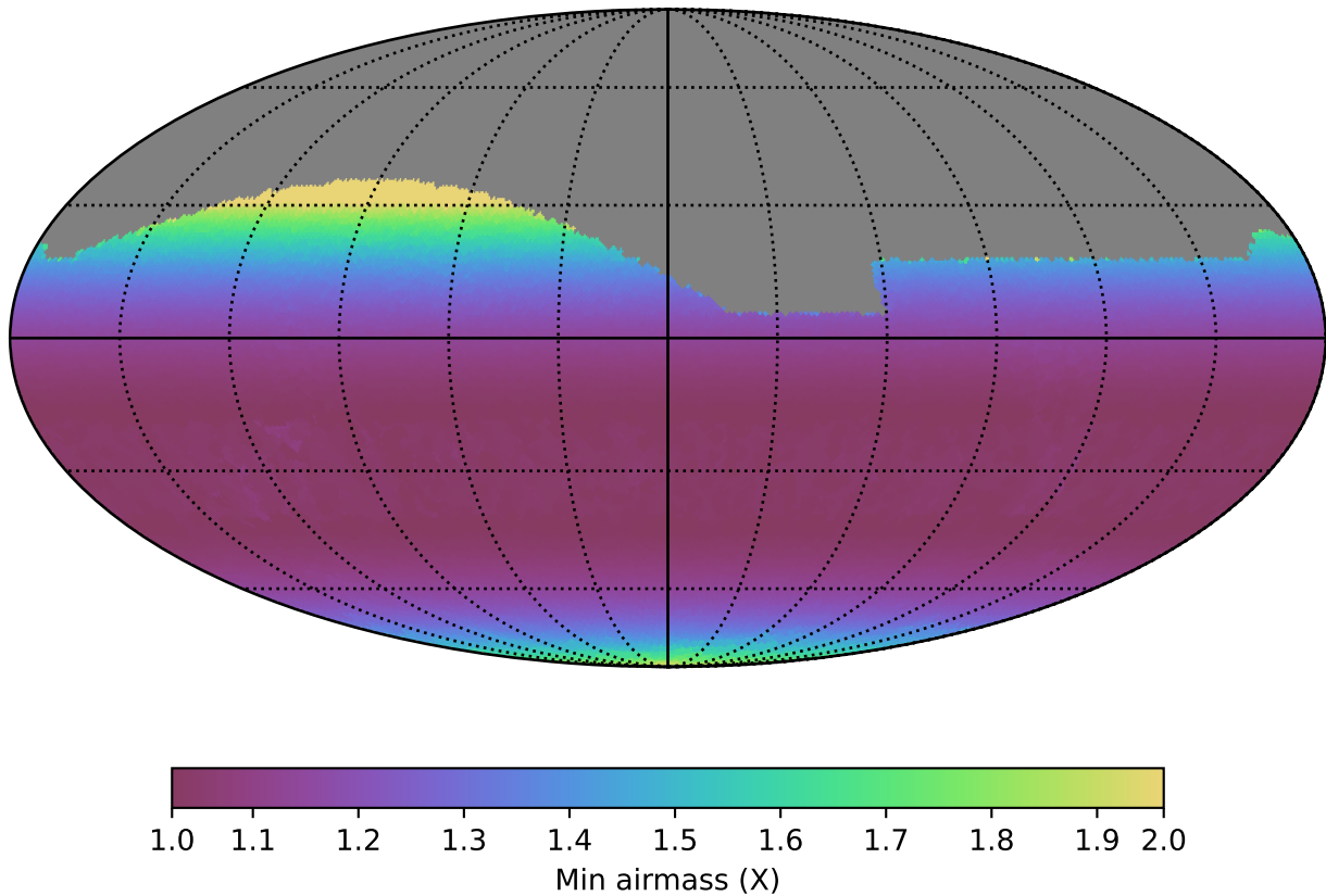
extra_ss_neo4_v3.4_10yrs All sky g band: Min airmass
