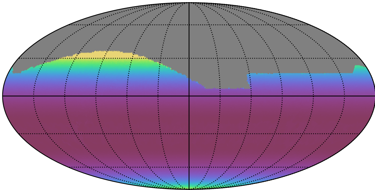
extra_ss_neo4_v3.4_10yrs All sky all bands: Min airmass
